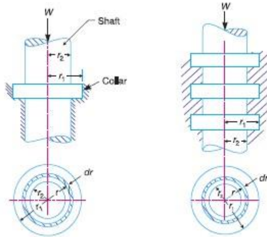
(a) Single collar bearing (b) Multiple collar bearing.
